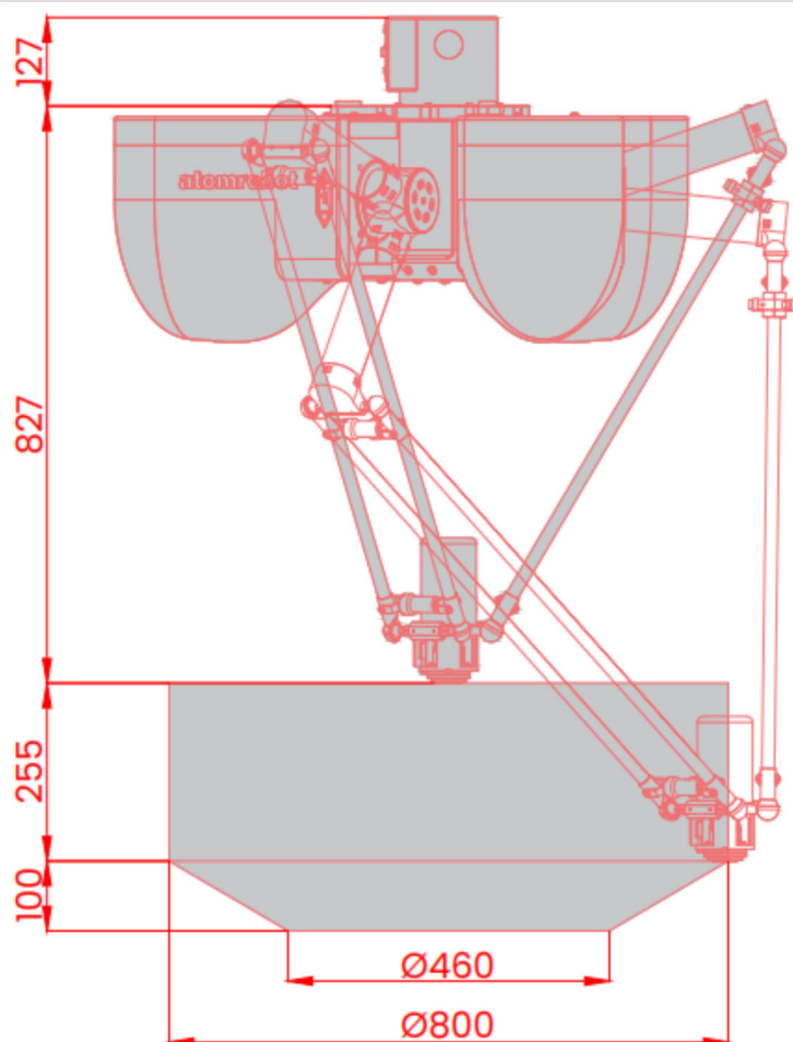
外形尺寸及运动范围 Outline dimensions and Working range (mm)
